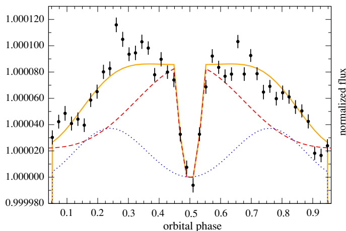
Figure 3. Phase-folded Kepler light curve with the best-fit model (solid curve). Also shown are the component stellar-only ellipsoidal model (dotted) and the planet-only model (offset by +1; dashed). Both the data and models have been cast into 30 minute bins.
